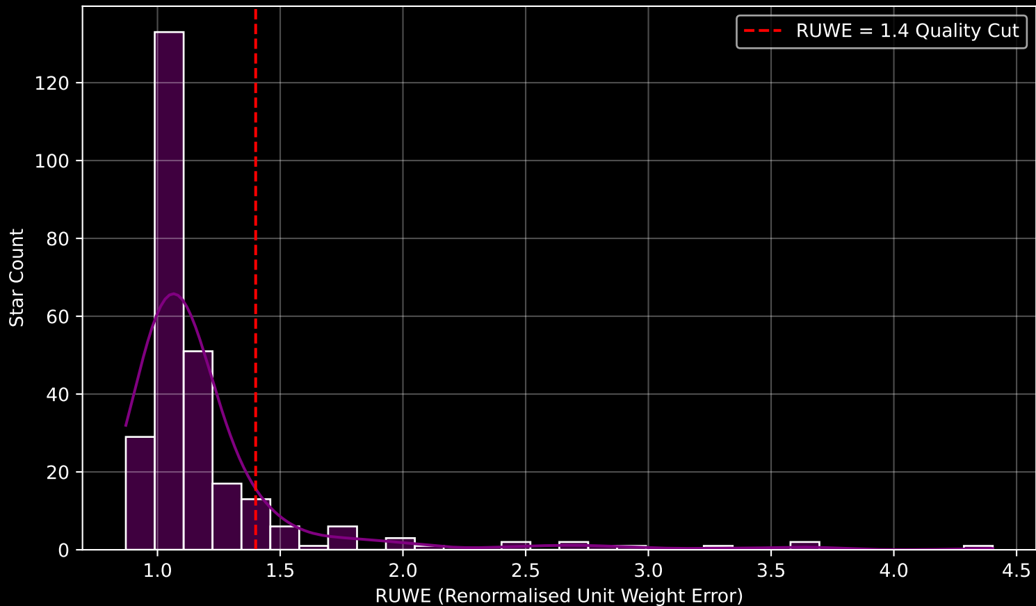
GALAH DR4 Field [9218] RUWE Distribution (n= 270)
