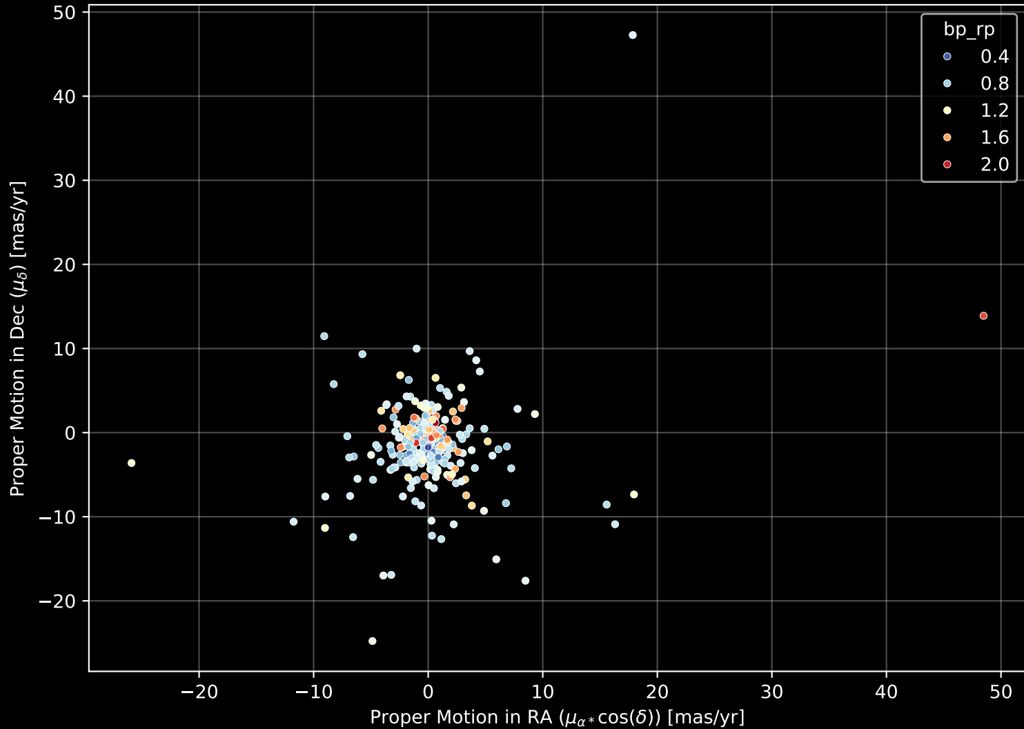
GALAH DR4 Field: [9218] Proper Motion Diagram (n= 279)
