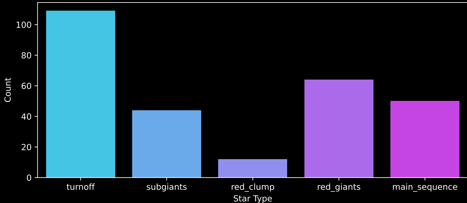
GALAH DR4 Field: [9218] Count plot of Star Type
